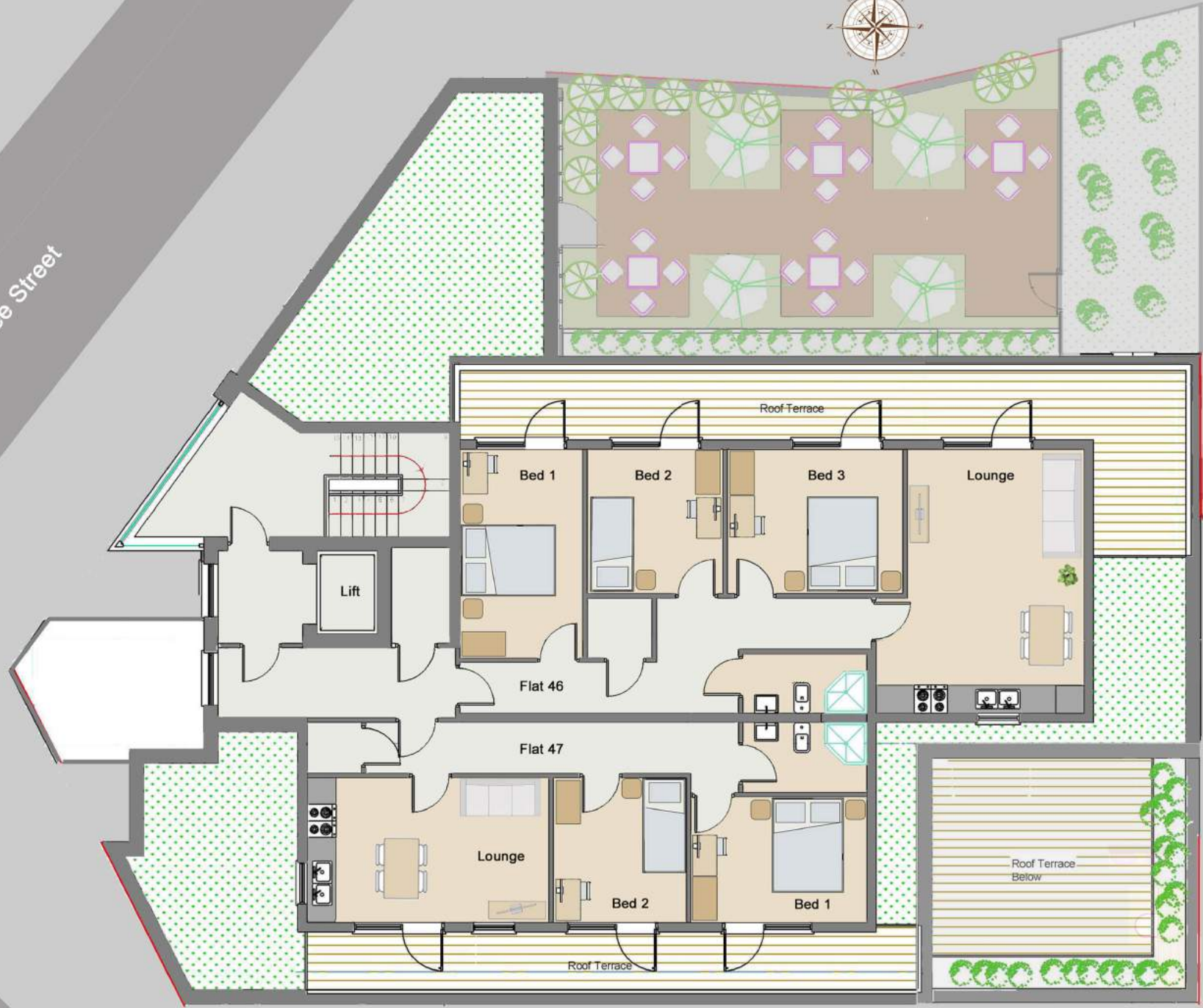
PROPOSED 6TH FLOOR PLAN
